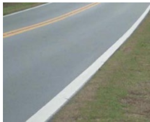
Wider Edge Lines (source: FHWA)
